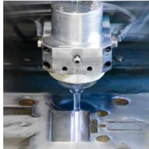
Wire EDM
